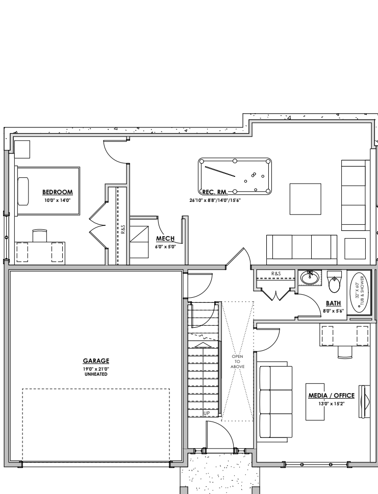
LOWER FLOOR
