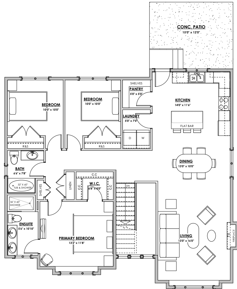
MAIN FLOOR
